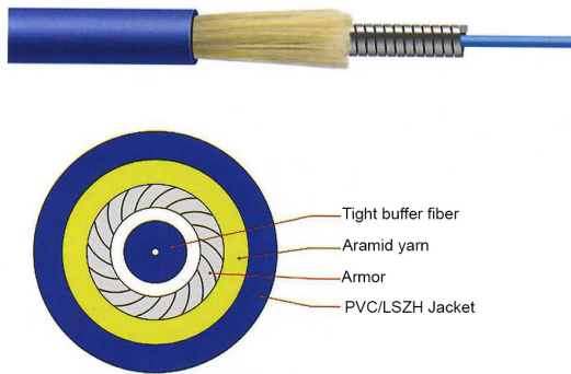
Simplex armoured cable
