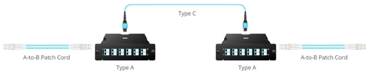
Connectivity Method C for duplex signals
