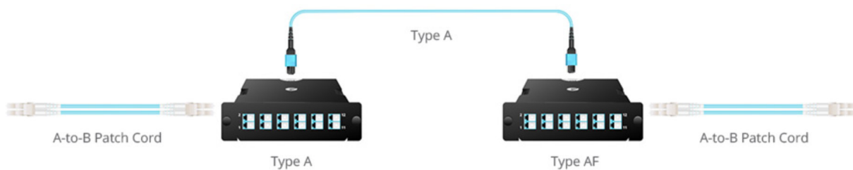
Connectivity Method A for duplex signals
