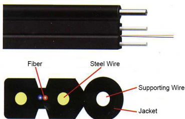
outdoor self-support drop cable
