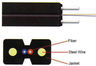
Indoor drop cable
