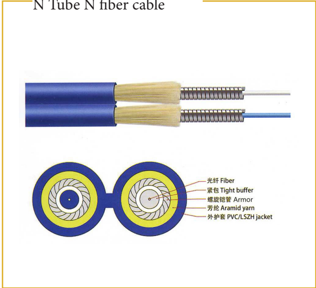
N Tube N fiber cable
